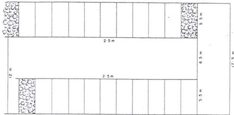
90° PARKING
