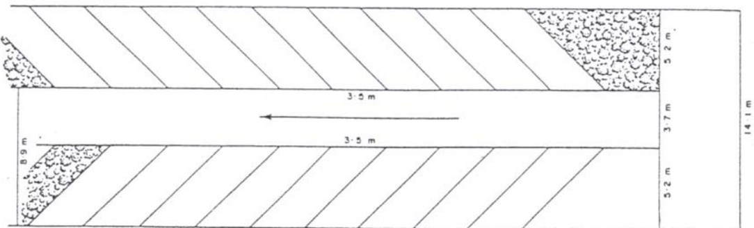
45° PARKING
