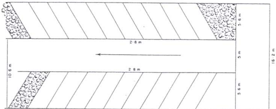
60° PARKING
